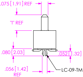
FIG 9 -EP (DIFFERENT AS SHOWN, OTHERWISE SAME AS FIG 1.)
