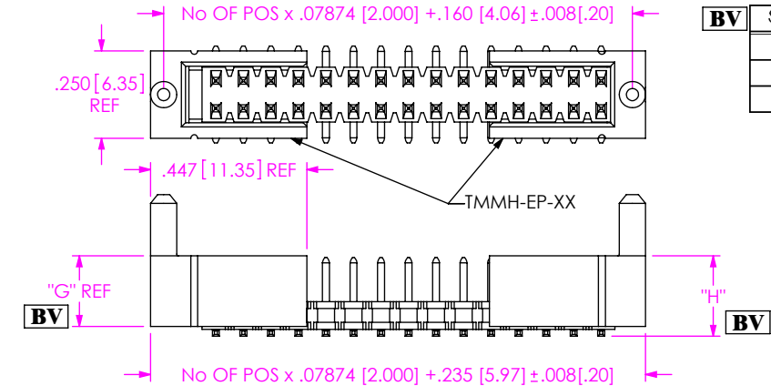
FIG 10 -EP-LC (DIFFERENT AS SHOWN, OTHERWISE SAME AS FIG 1.)
