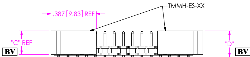
FIG 4 -ES (DIFFERENT AS SHOWN, OTHERWISE SAME AS FIG 1.)
