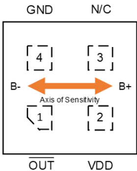
Figure 4: CT8131 4-Lead LGA Package with Digital Output (Top View)
