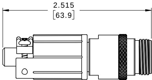
ASSEMBLED VIEW FOR CUSTOMER REFERENCE ONLY
