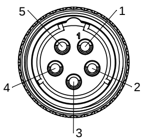
WIRE VIEW SF8382-5SG-5XX
