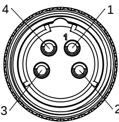
WIRE VIEW SF8382-4SG-5XX
