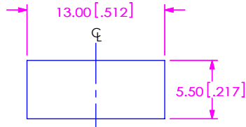
SUGGESTED PANEL CUTOUT DIMENSIONS
