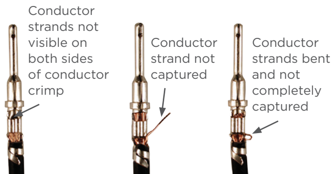
Unacceptable Crimps
