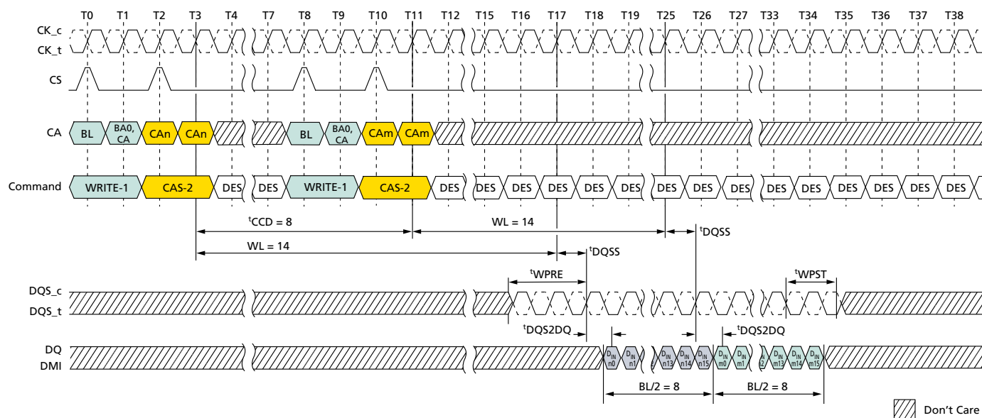
Figure 56: Seamless WRITE: t_{\text{CCD}} = \text{MIN} , 1.5n\text{CK} Postamble
