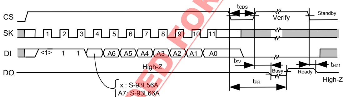
Figure 13 Data Erase Timing (S-93L56A, S-93L66A)
