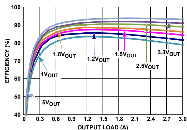
FIGURE 6. EFFICIENCY vs LOAD, 12V IN CCM
