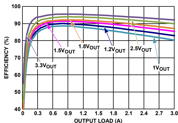
FIGURE 4. EFFICIENCY vs LOAD, 5V IN CCM
