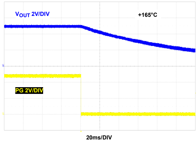
FIGURE 40. OVER-TEMPERATURE PROTECTION
