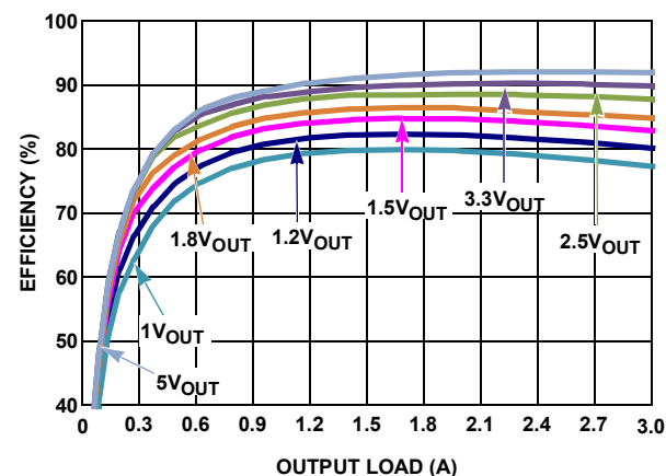
FIGURE 8. EFFICIENCY vs LOAD, 18V IN CCM
