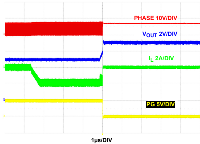
FIGURE 39. OVERVOLTAGE PROTECTION
