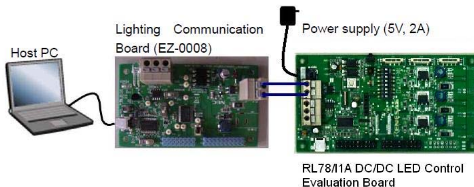
Figure 50: System Configuration for DALI Control
