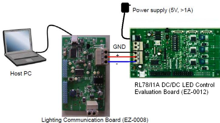
Figure 47: System Configuration for DMX512 Control
