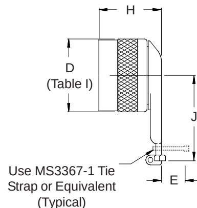
90° ROTATABLE COUPLING
