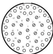
22-39 27 contacts size 20 12 contacts size 16
