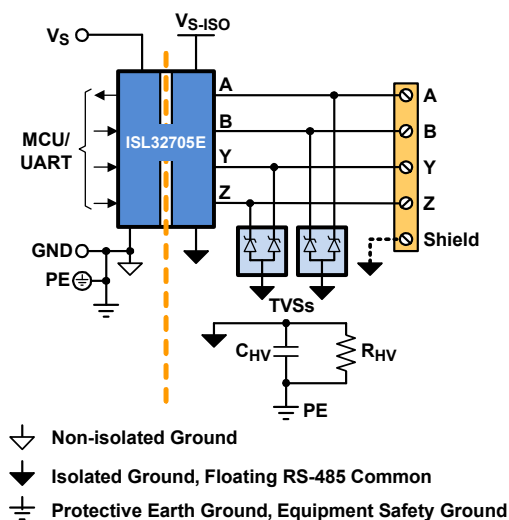
Figure 10. Transient Protection for ISL32705E
