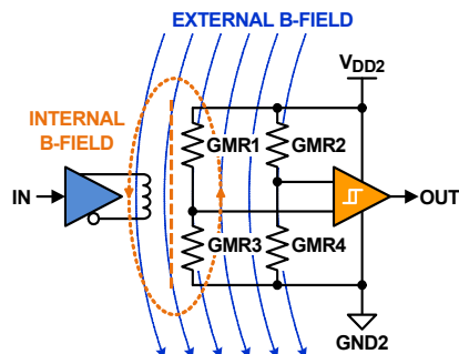
Figure 5. Single Channel GMR Isolator
