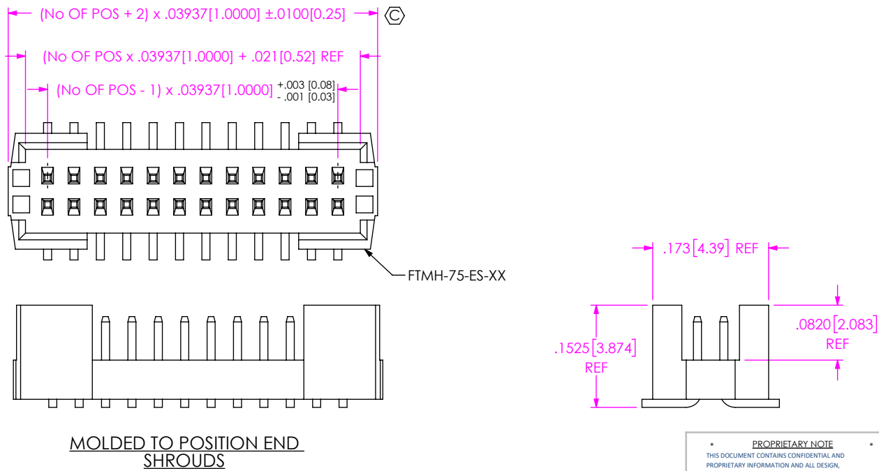
FIG 2 -ES: END SHROUDS FTMH-112-02-X-DV-ES SHOWN (DIFFERENT AS SHOWN, OTHERWISE SAME AS FIG 1)
