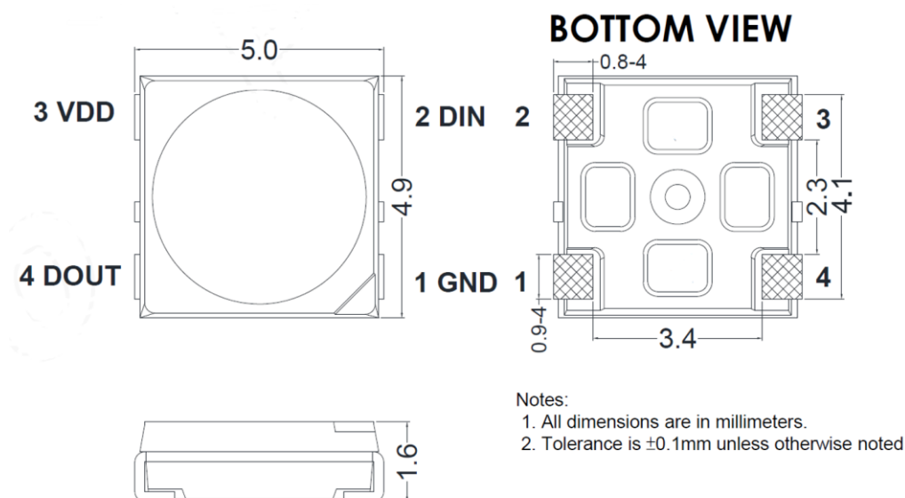
Figure 1. IN-PI55QATPRPGPBPW-XX Package Outline Dimensions
