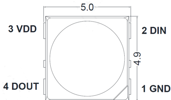
Figure 2. IN- PI55QATPRPGPBPW-XX Pin Configuration
