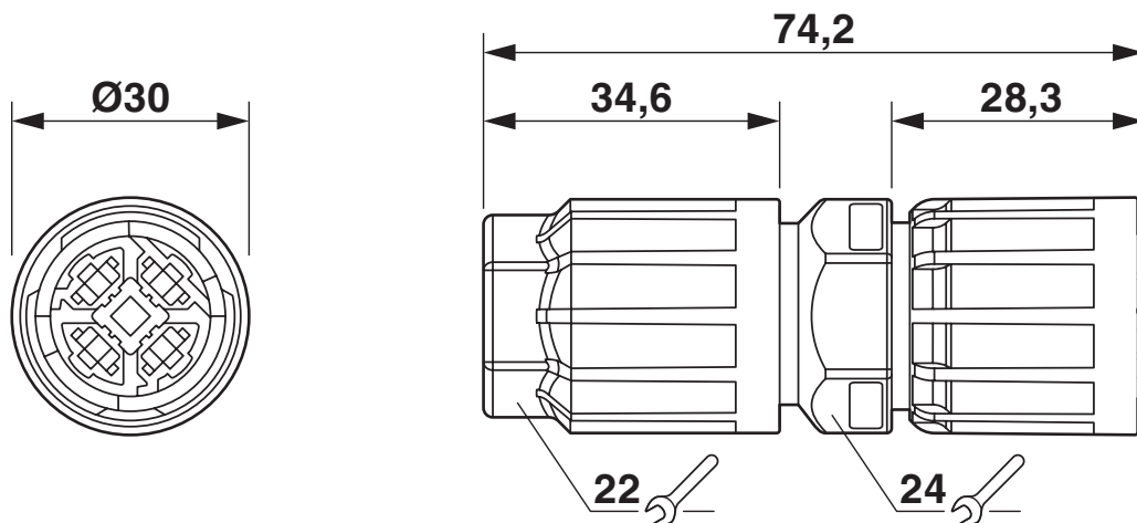
Dimensional drawing
