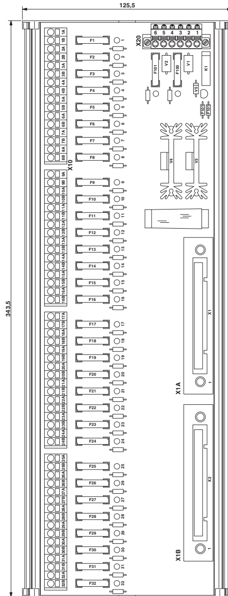
Dimensional drawing
