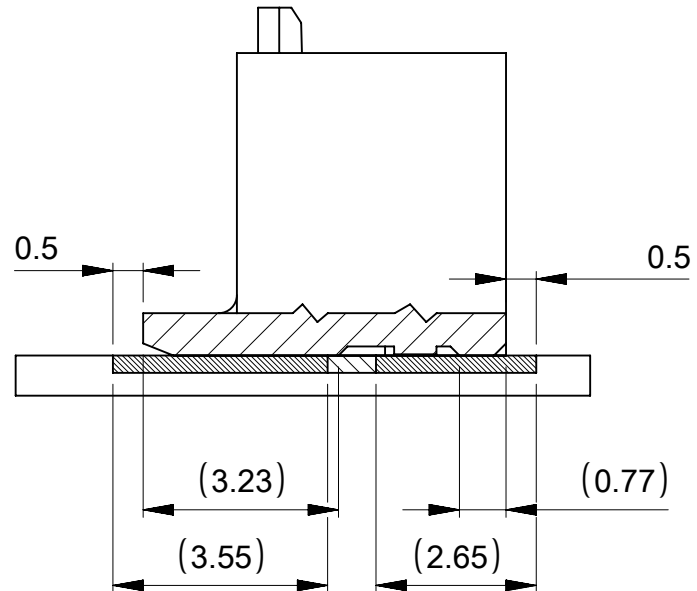
SECTION Z-Z
