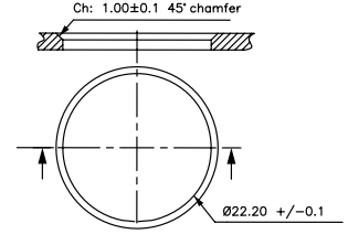
IP69K PANEL CUT OUT
