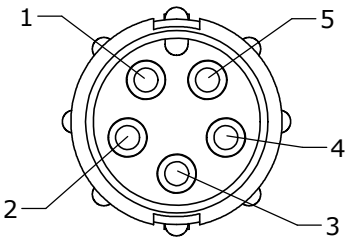
FACE VIEW 8382-5PG-5XX
