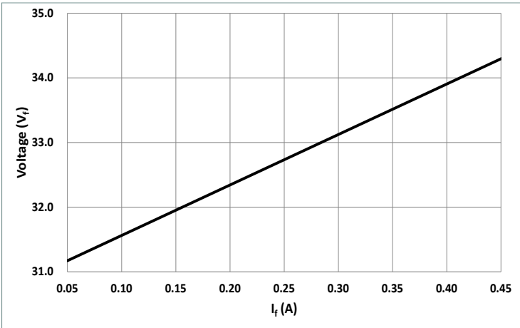
Forward Current vs. Forward Voltage @ 85°C
