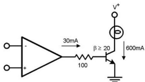
Lamp Driver
