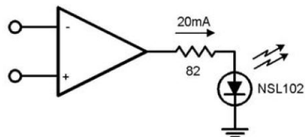
LED Driver
