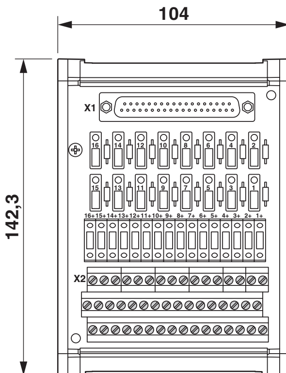
Dimensional drawing
