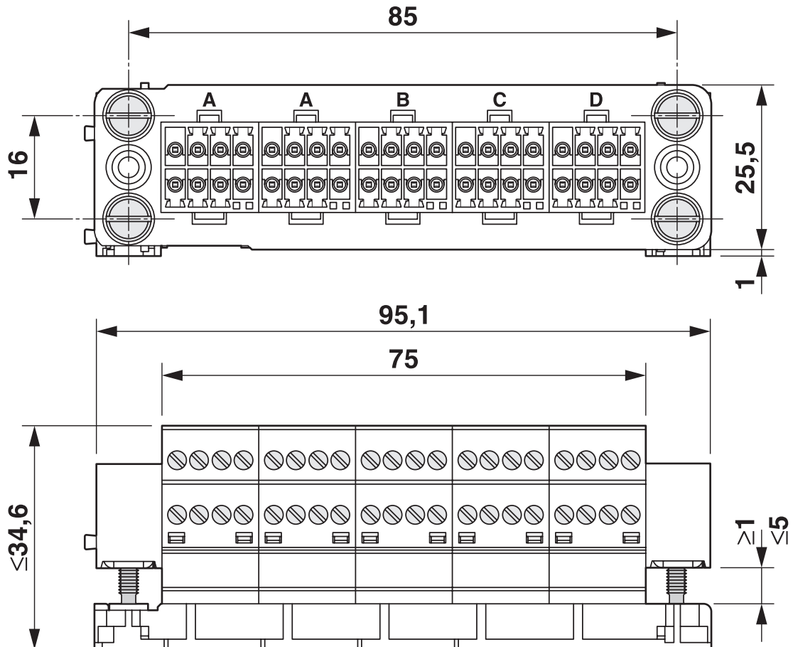
Dimensional drawing
