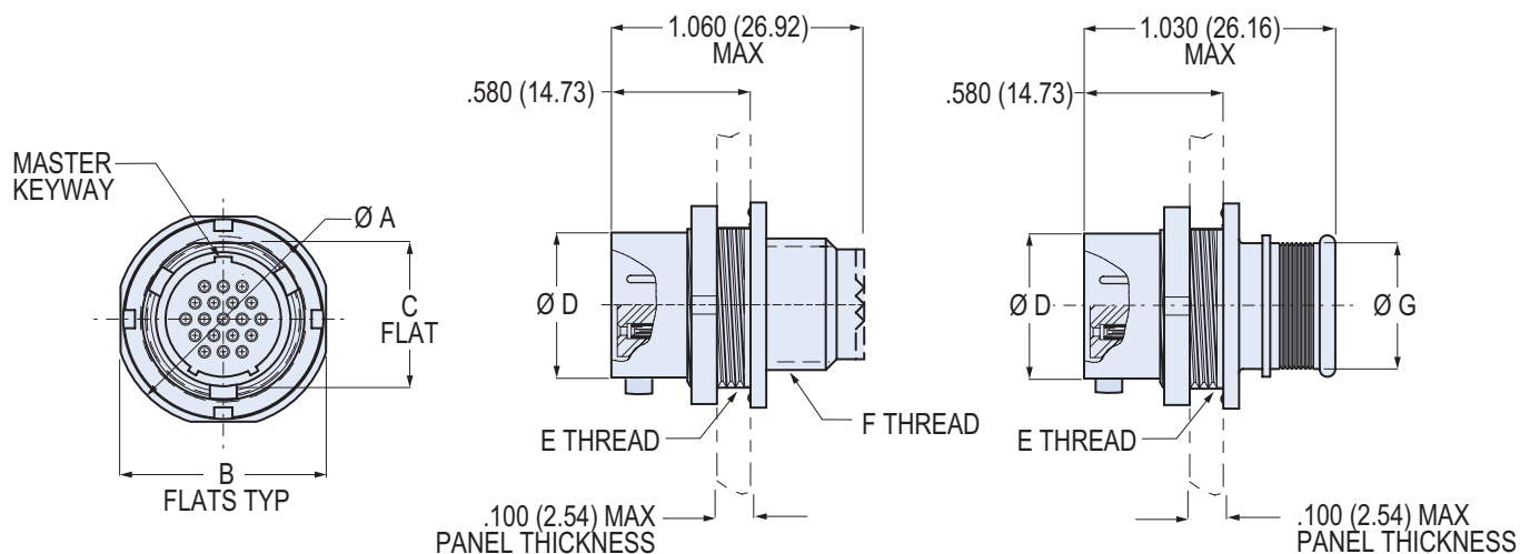
Accessory Thread 803-004
