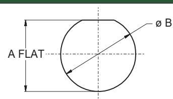
Series 801 Jam-Nut Panel Cutout
