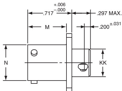
Commercial LJT02RE-XX-XXX
