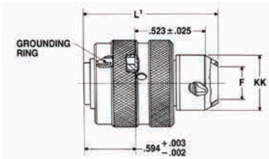
Commercial LJT06P-XX-XXX
