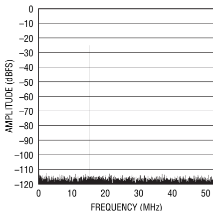
LTC2207-14: 64K Point FFT, f_{IN} = 15.1\text{MHz} , -25\text{dBFS} , PGA = 0, RAND "On", Dither "On"
