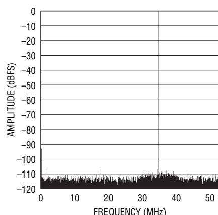
LTC2207-14: 32K Point FFT, f_{IN} = 70.24\text{MHz} , -1\text{dBFS} , PGA = 0, RAND "On", Dither "Off"
