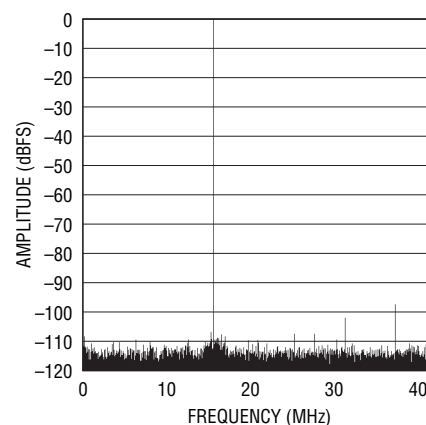
LTC2206-14: 32K Point FFT, f_{IN} = 14.86\text{MHz} , -1\text{dBFS} , \text{PGA} = 0 , \text{RAND} = \text{"On"} , Dither "Off"
