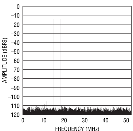
LTC2207-14: 32K Point 2-Tone FFT, f_{IN} = 14.87\text{MHz} and 18.56\text{MHz} , -15\text{dBFS} , PGA = 0, RAND "On", Dither "Off"
