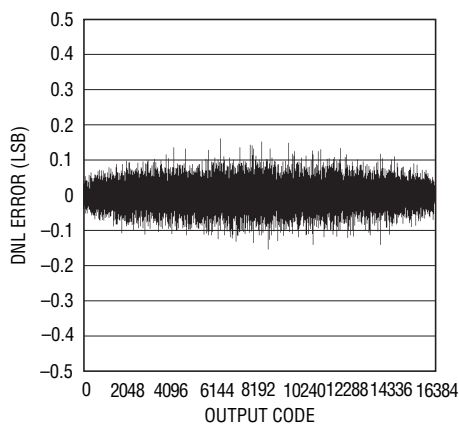
LTC2206-14: Differential Nonlinearity (DNL) vs Output Code
