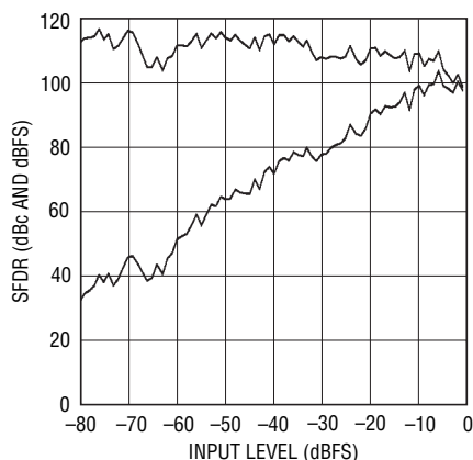
LTC2207-14: SFDR vs Input Level, f_{IN} = 15.1\text{MHz} , PGA = 0, RAND "On", Dither "Off"
