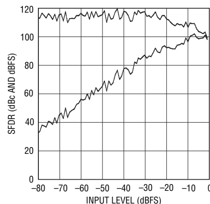
LTC2207-14: SFDR vs Input Level, f_{IN} = 15.1\text{MHz} , PGA = 0, RAND "On", Dither "On"
