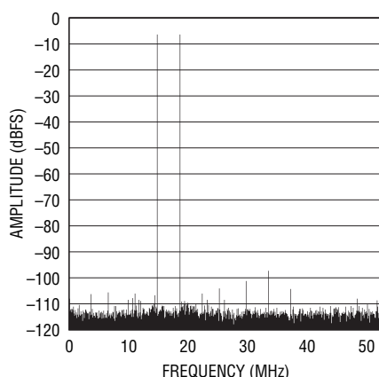
LTC2207-14: 32K Point 2-Tone FFT, f_{IN} = 14.87\text{MHz} and 18.56\text{MHz} , -7\text{dBFS} , PGA = 0, RAND "On", Dither "Off"
