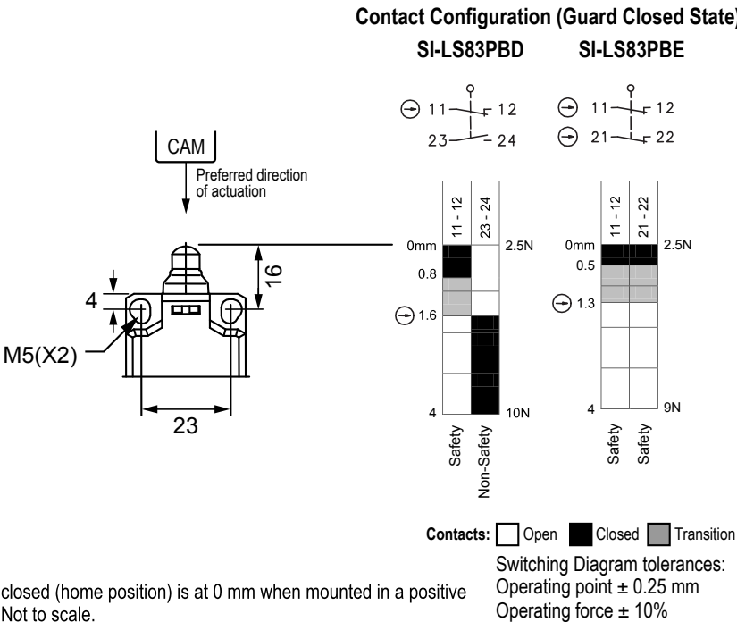
SI-LS83PBx Switching Diagrams
