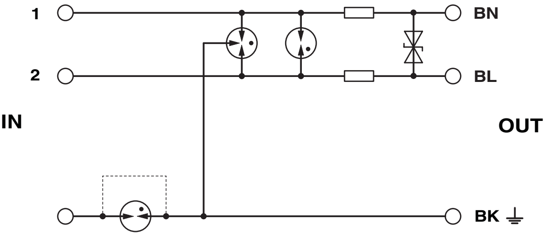
Circuit diagram
