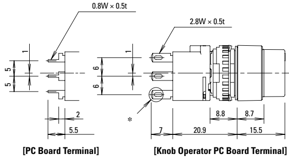
[SPDT/DPDT]
