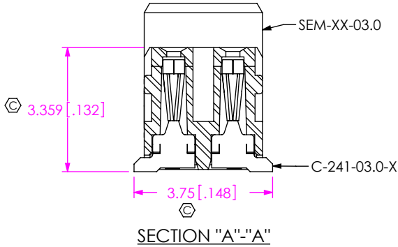
FIG 1 SEM-110-02-03.0-XX-D SHOWN
