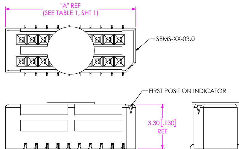
FIG 6 SEMS-110-02-03.0-XX-D SHOWN (DIFFERENT AS SHOWN, OTHERWISE SAME AS FIG 1)
