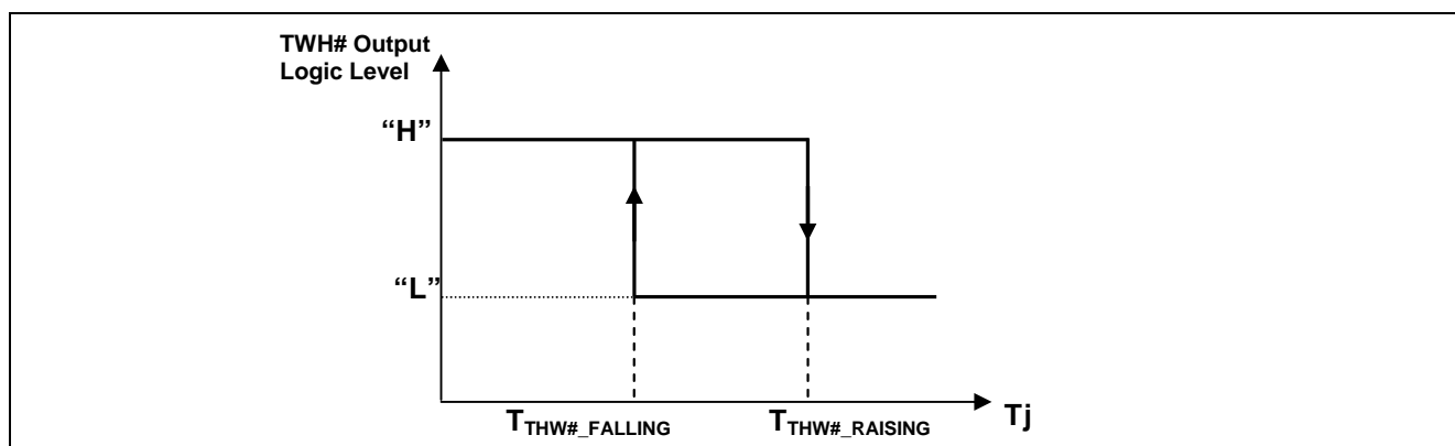
Figure 5 Thermal warning
