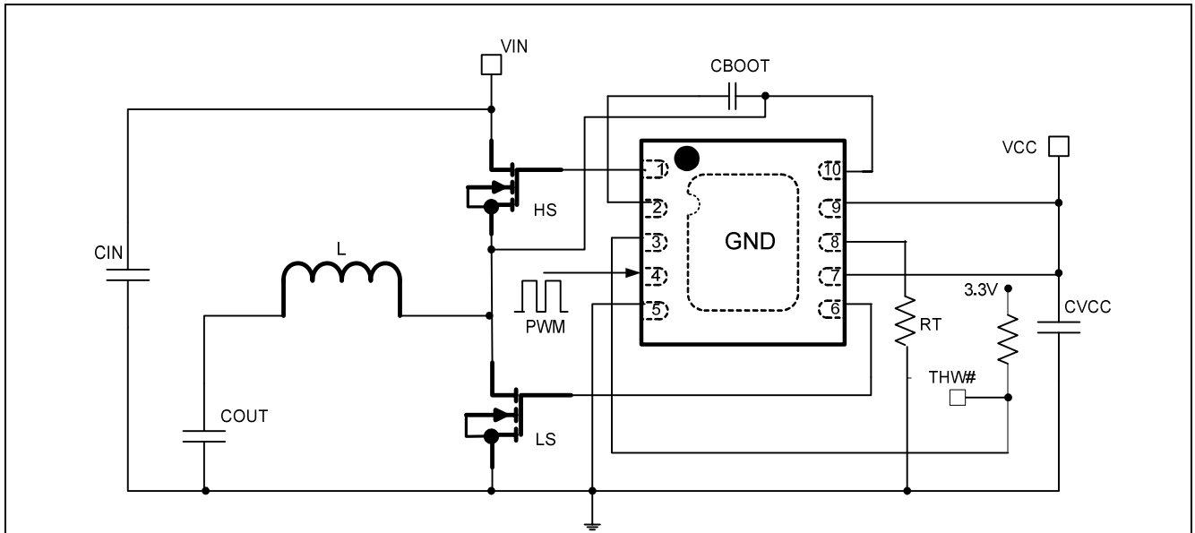
Figure 6 Pin interconnection outline (transparent top view)
