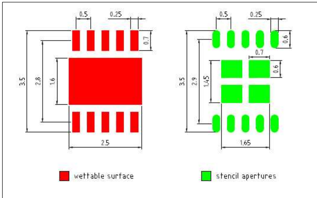
Figure 9 Footprint
