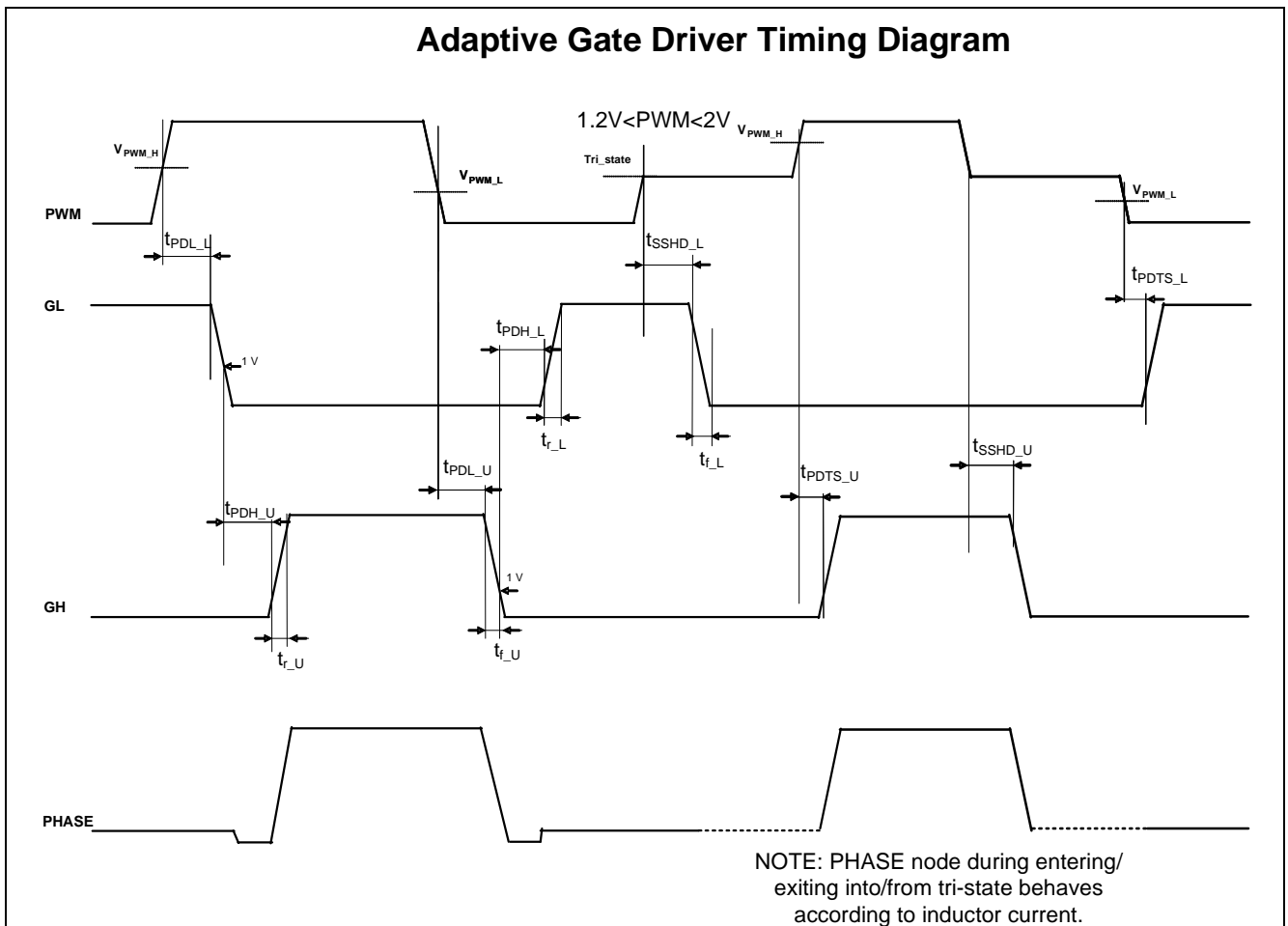
Figure 7 Adaptive gate driver timing diagram
