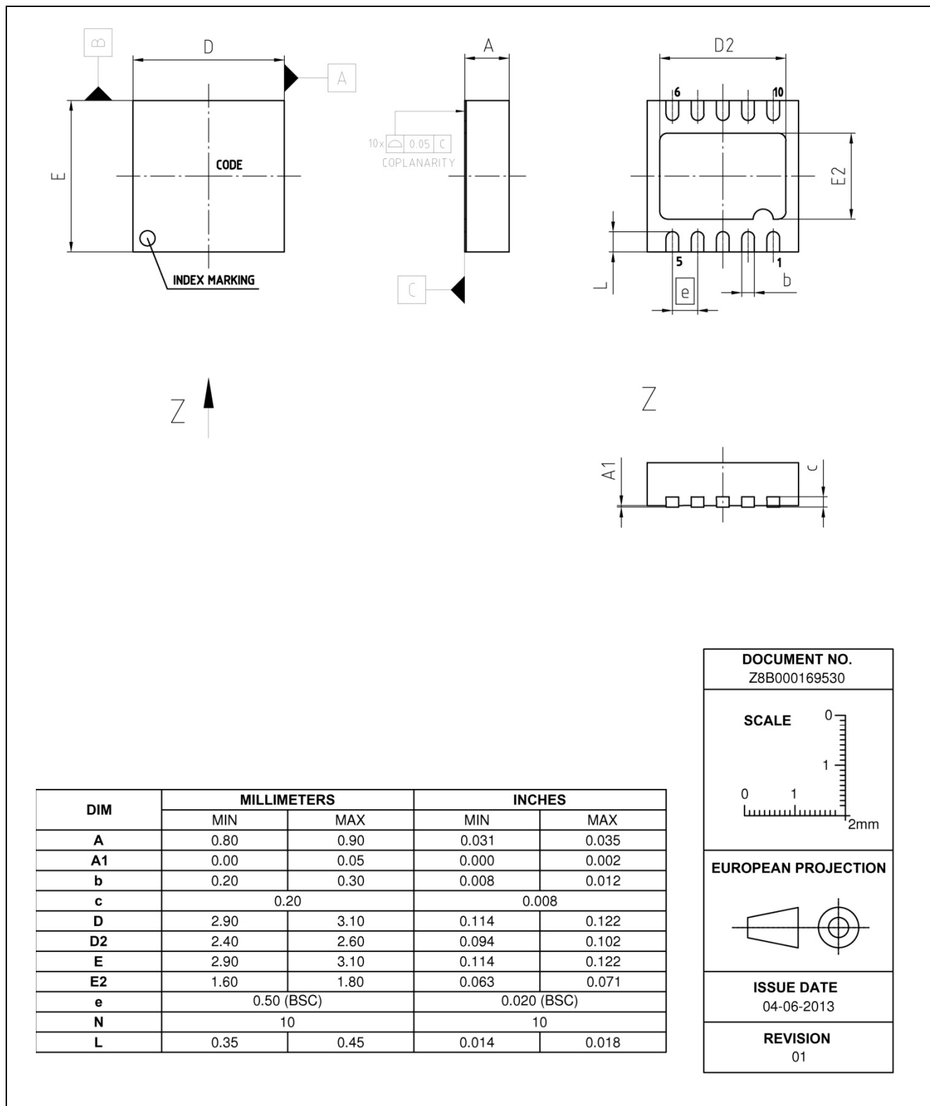
Figure 8 Mechanical dimensions
