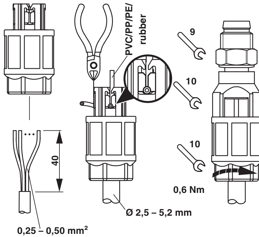
Functional drawing
