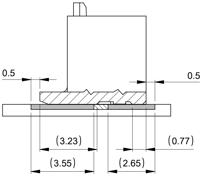
SECTION Z-Z
