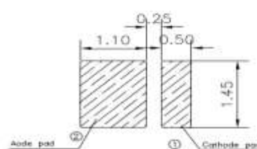
Recommended soldering pattern layout
