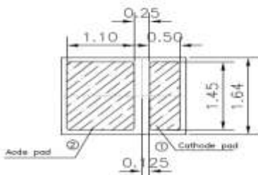
Component bottom view
