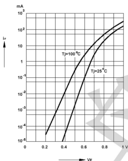
Forward characteristics
