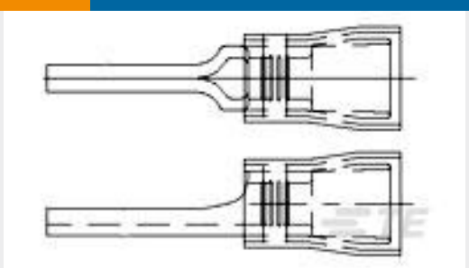
TE Part #696274-2 TERM, WIRE PIN, PIDG, 16-14, T&R
