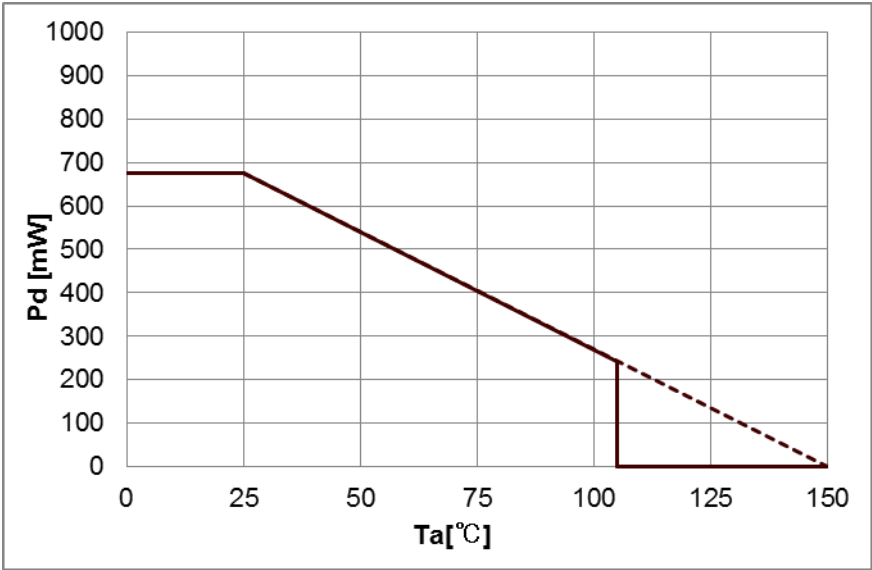
Figure 37, SSOP6 Thermal Reduction Characteristics
