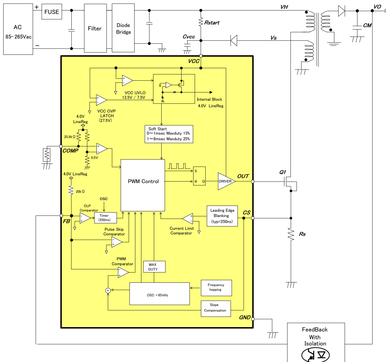
Figure 4. Block Diagram
