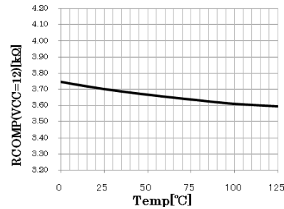
Figure 31, RCOMP (VCC=12)
