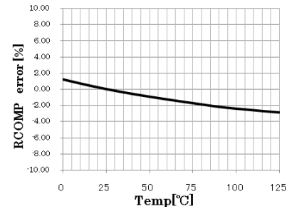
Figure 32, RCOMP Error
