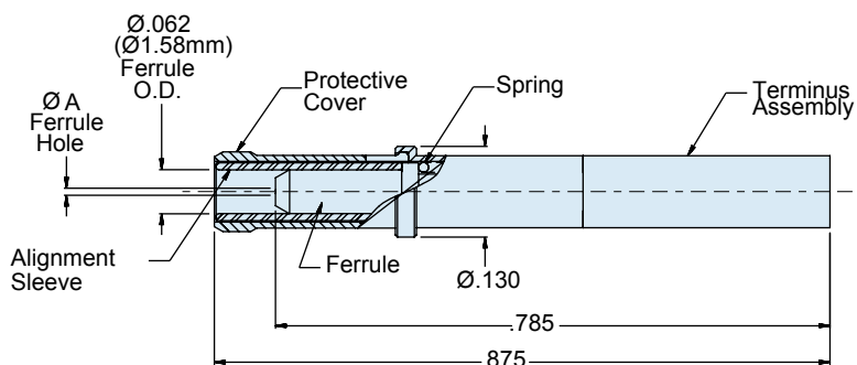
181-075 Socket Terminus
