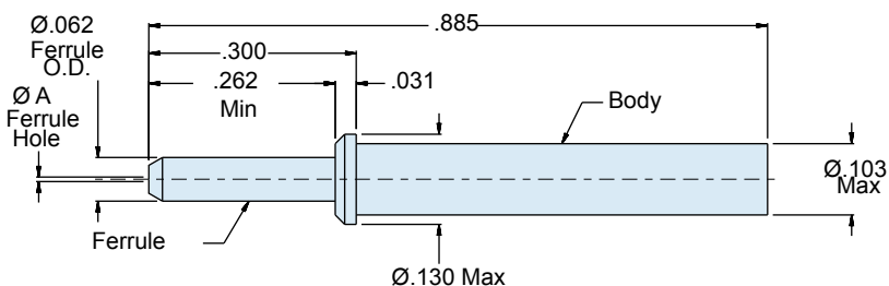
181-057 Pin Terminus
