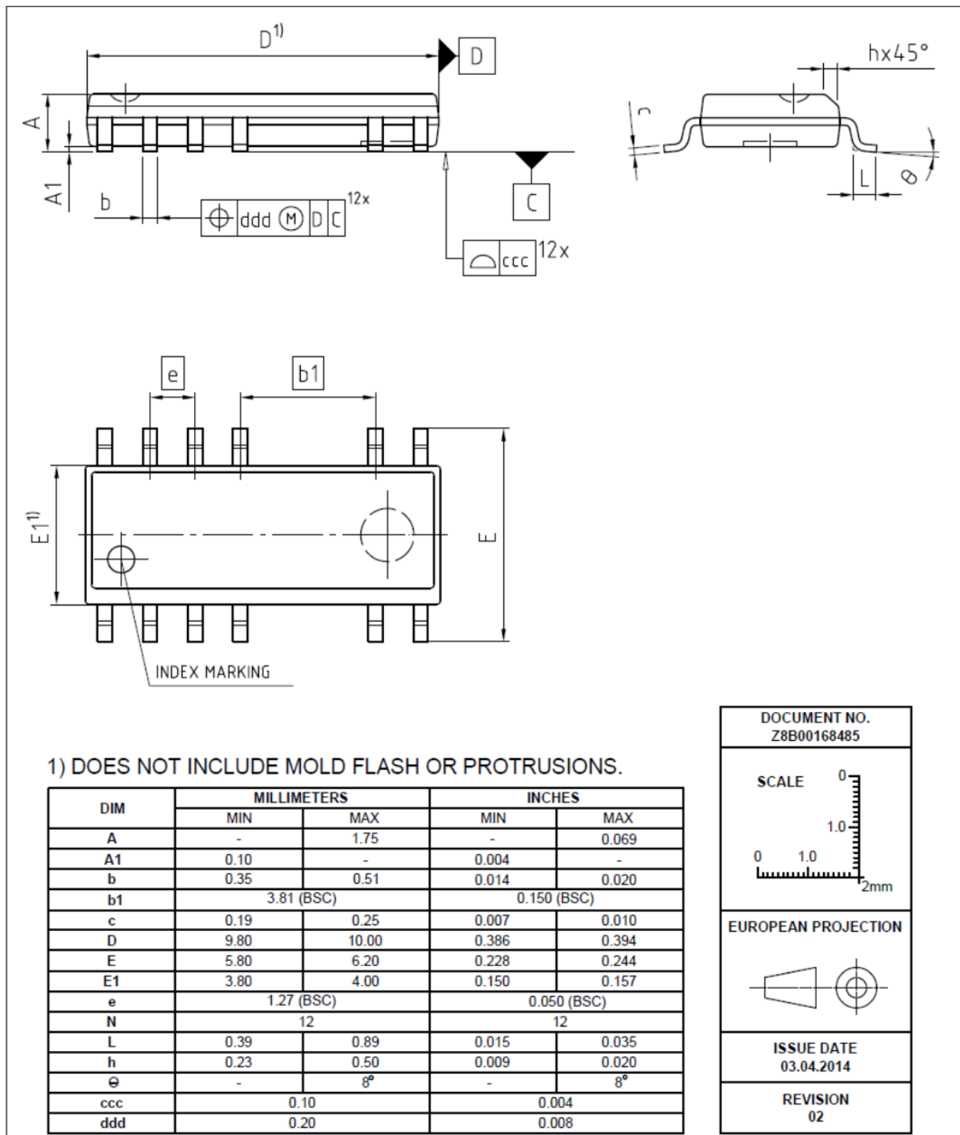
Figure 35 PG-DSO-12
