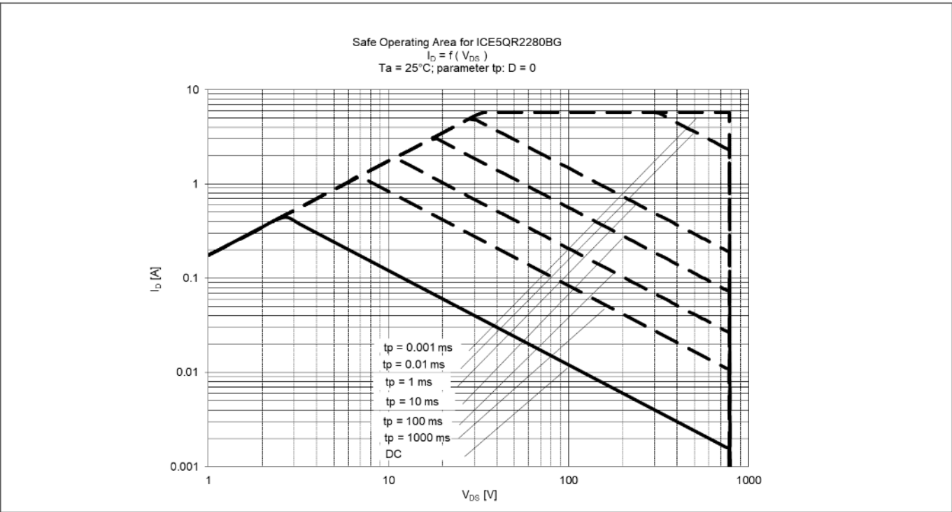
Figure 15 Safe Operating Area (SOA) curve for ICE5QR2280BG
