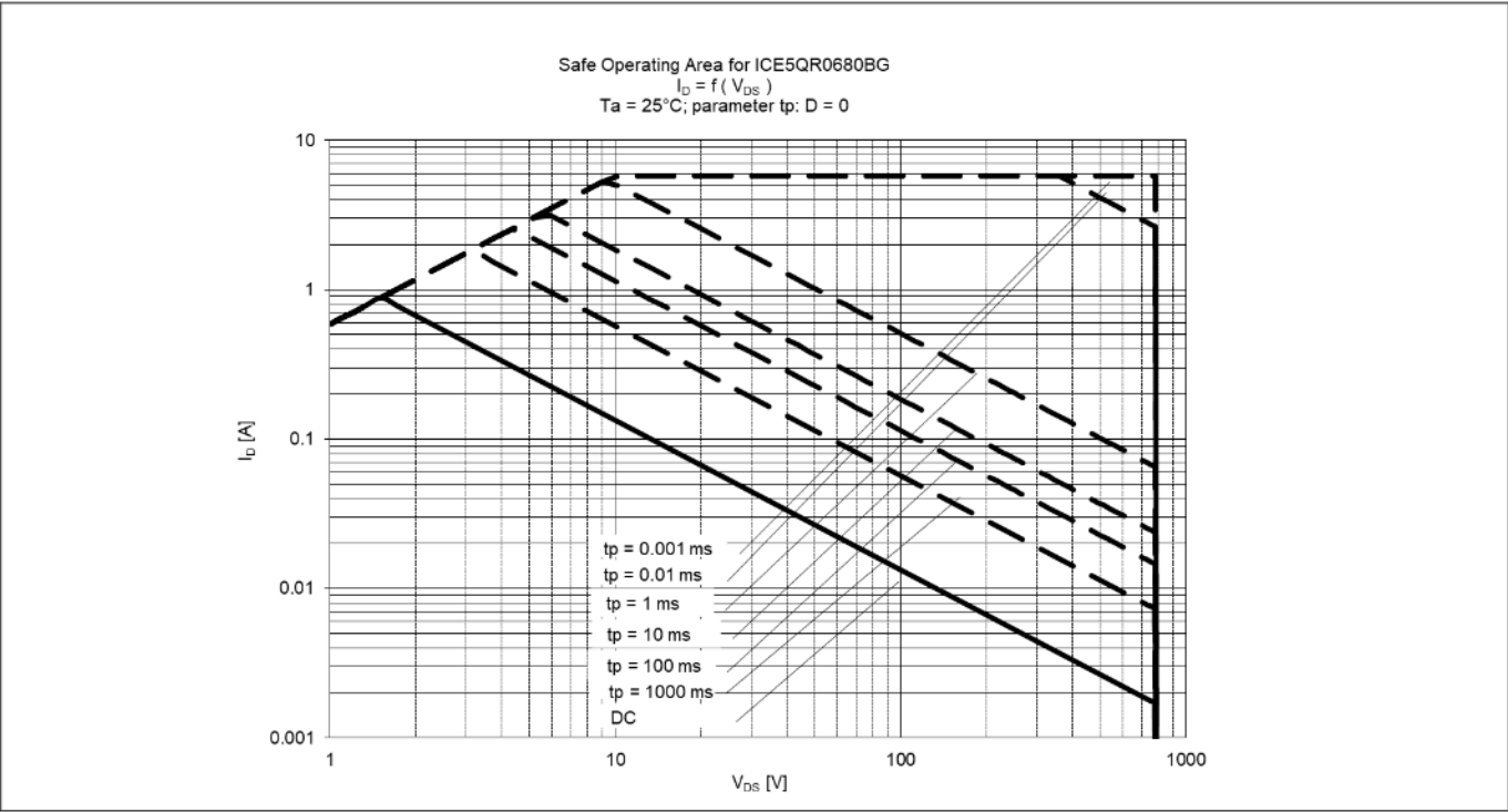
Figure 17 Safe Operating Area (SOA) curve for ICE5QR0680BG
