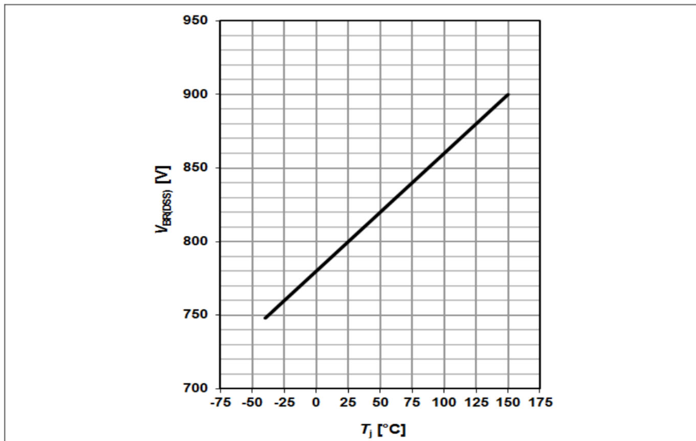
Figure 22 Drain-source breakdown voltage ICE5QRxx80BG; V_{BR(DSS)} = f(T_J) , I_D = 1 mA
