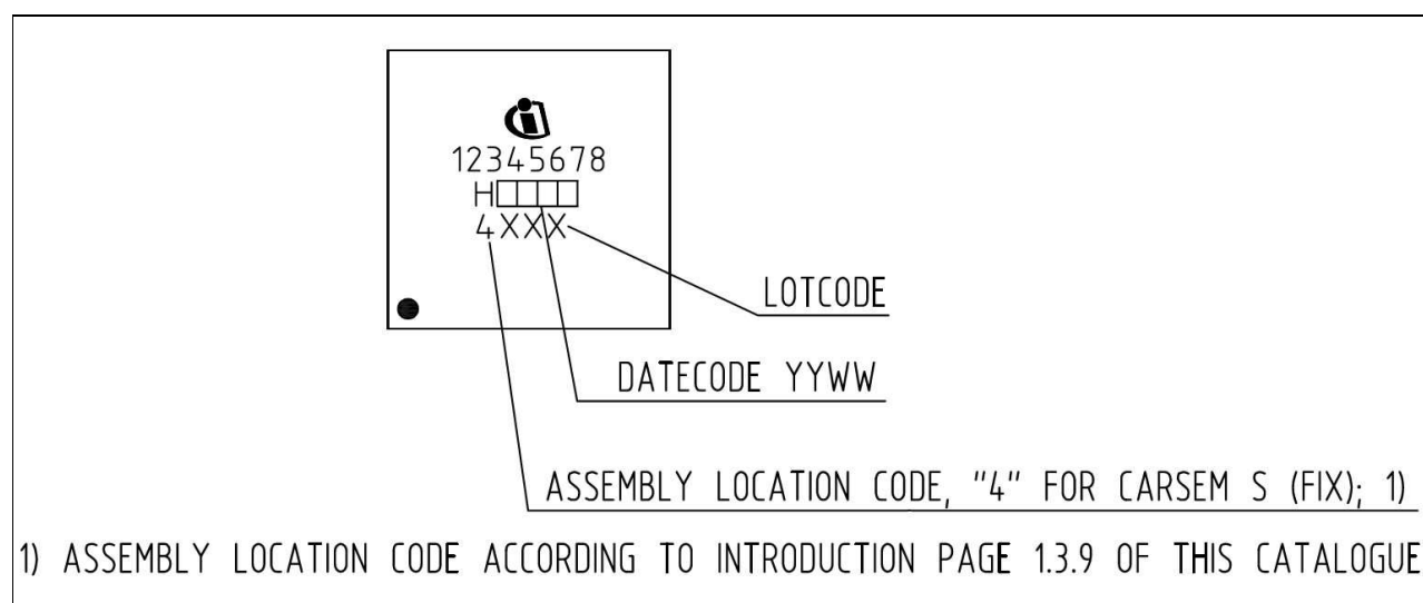
Figure 58 Part marking
