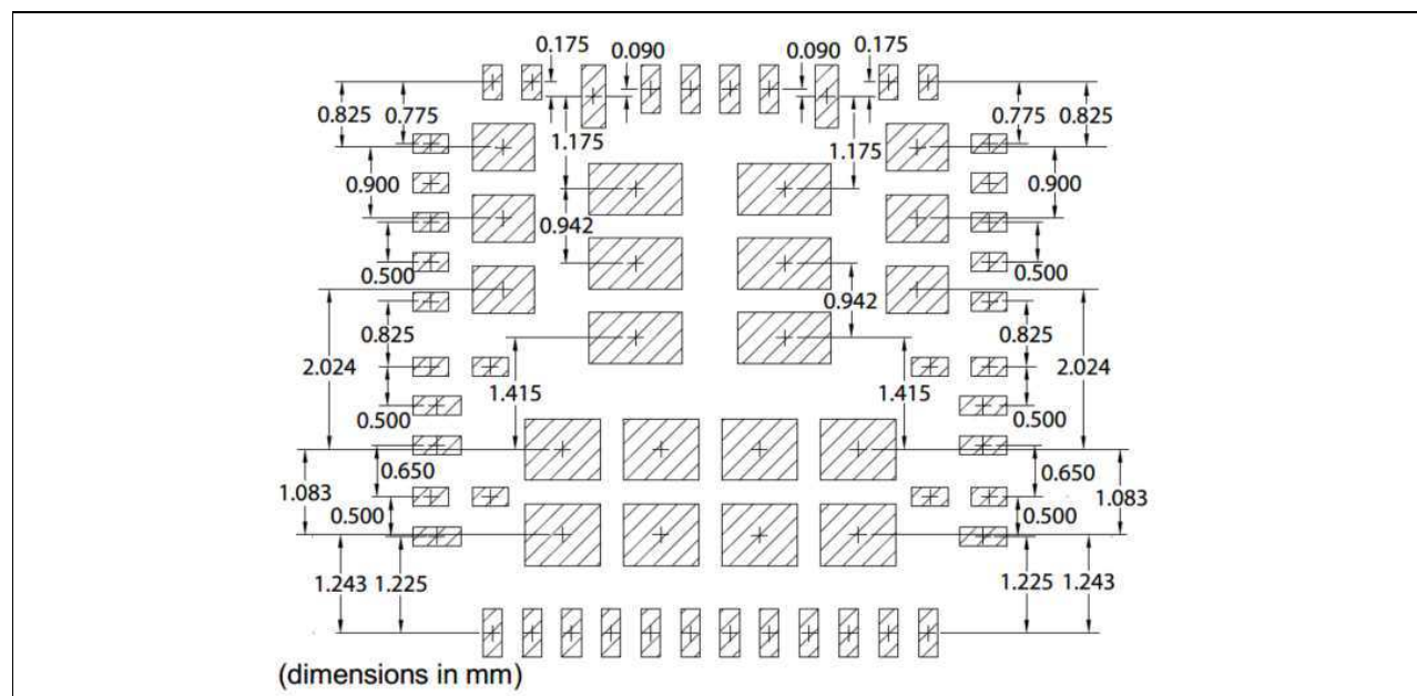
Figure 57 42-lead 7x7 stencil design_3
