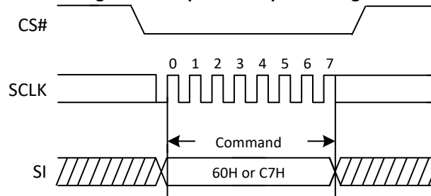
Figure 27. Chip Erase Sequence Diagram
