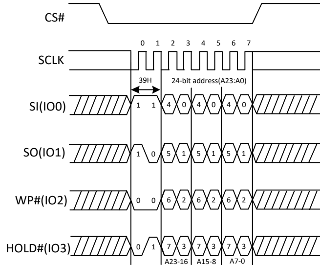
Figure 47d. Read Individual Block/Sector lock command Sequence Diagram
