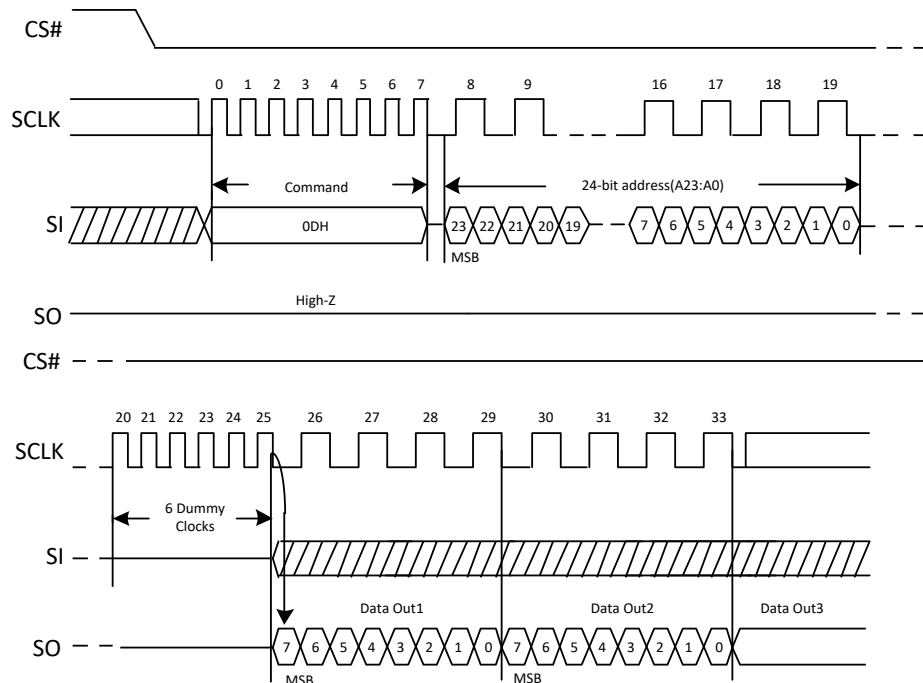
Figure 18. DTR Fast Read Instruction (SPI Mode)
