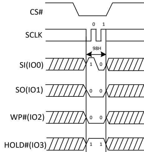
Figure 46c. The Global Block/Sector Unlock Sequence Diagram (QPI)
