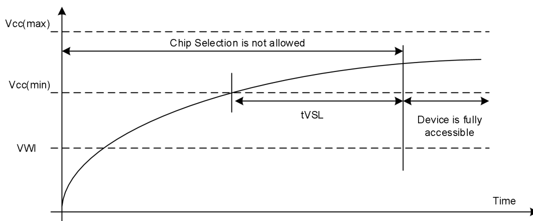
Figure26. Power-On Timing
