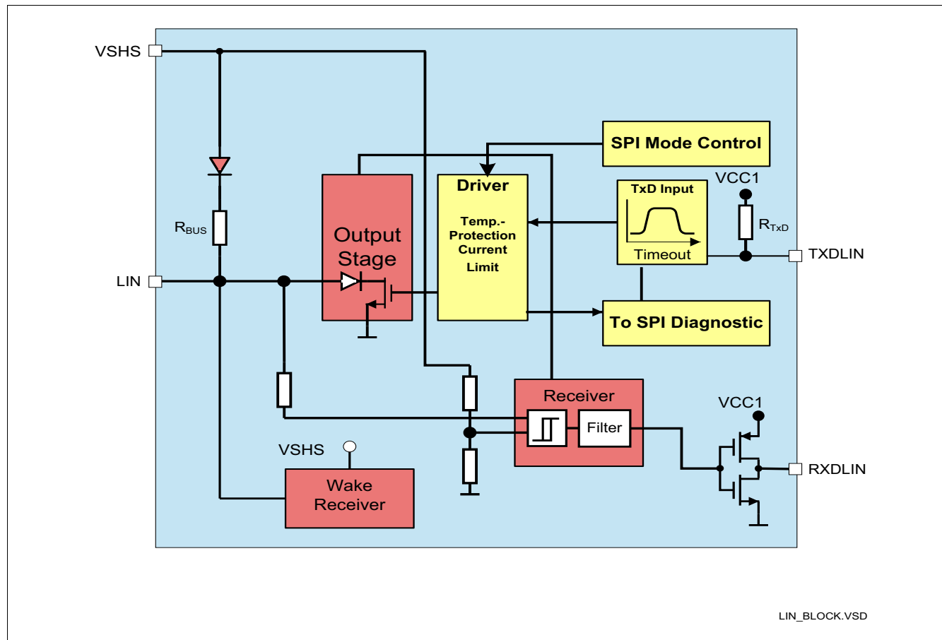
Figure 31 Block Diagram
