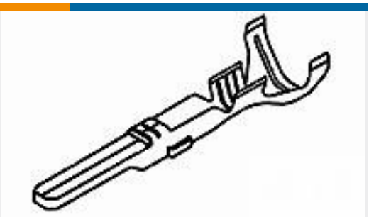
TE Part #881590-1 ECONOSEAL TAB .070
