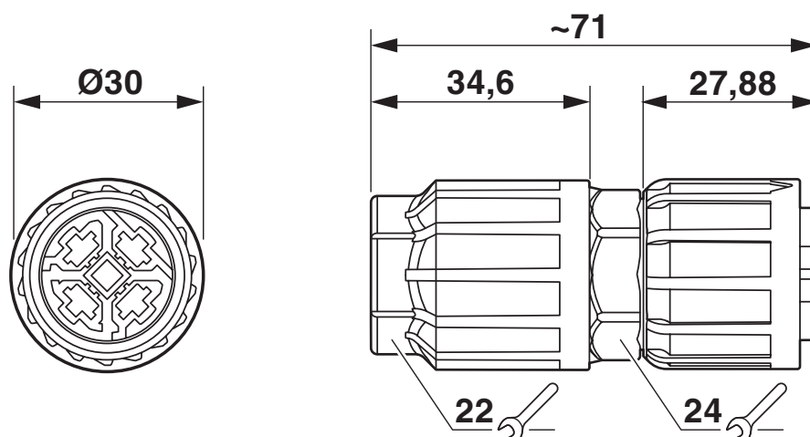
Dimensional drawing
