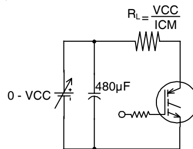
Pulsed Collector Current Test Circuit Fig. 20 - Pulsed Collector Current Test Circuit
