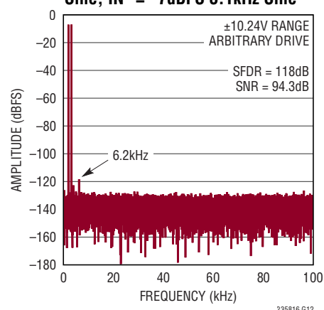
32k Point Arbitrary Two-Tone FFT f_{SMPL} = 200\text{kHz} , IN^+ = -7\text{dBFS } 2\text{kHz} Sine, IN^- = -7\text{dBFS } 3.1\text{kHz} Sine
