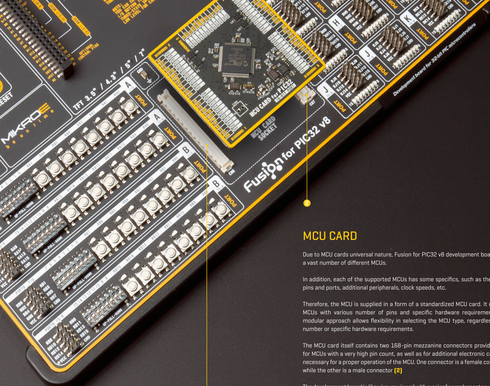
Figure 6: Main board with MCU card socket view
