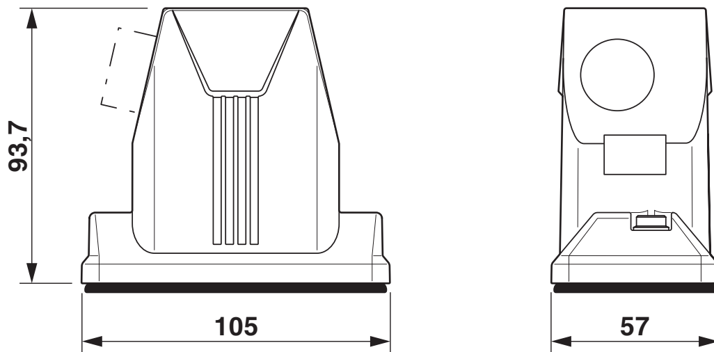
Dimensional drawing
